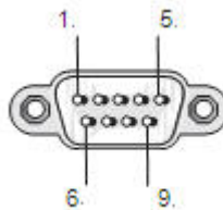
Figure 1: Serial Port Pin Definition (DB-9 DTE)
